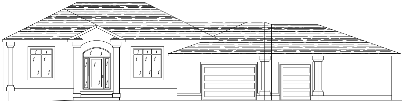
—FRONT ELEVATION—
